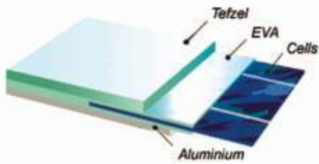
Laminated Solar Module Tefzel-Aluminium
