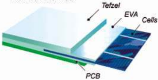
Laminated Solar Module Tefzel-PCB
